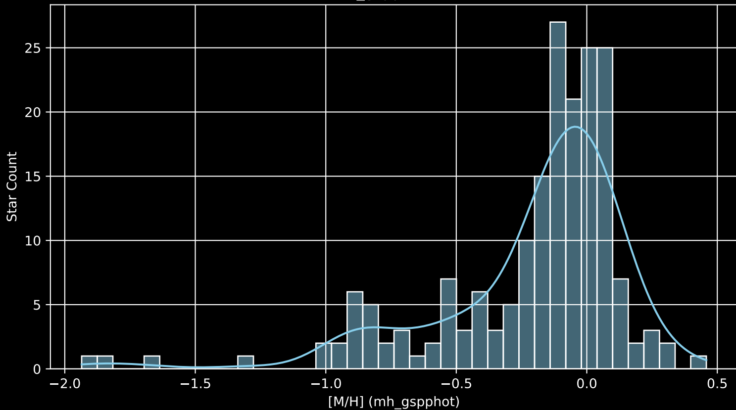
APOGEE DR17 Field: [173-04 [M/H] (mh_gspphot) (n= 189)
