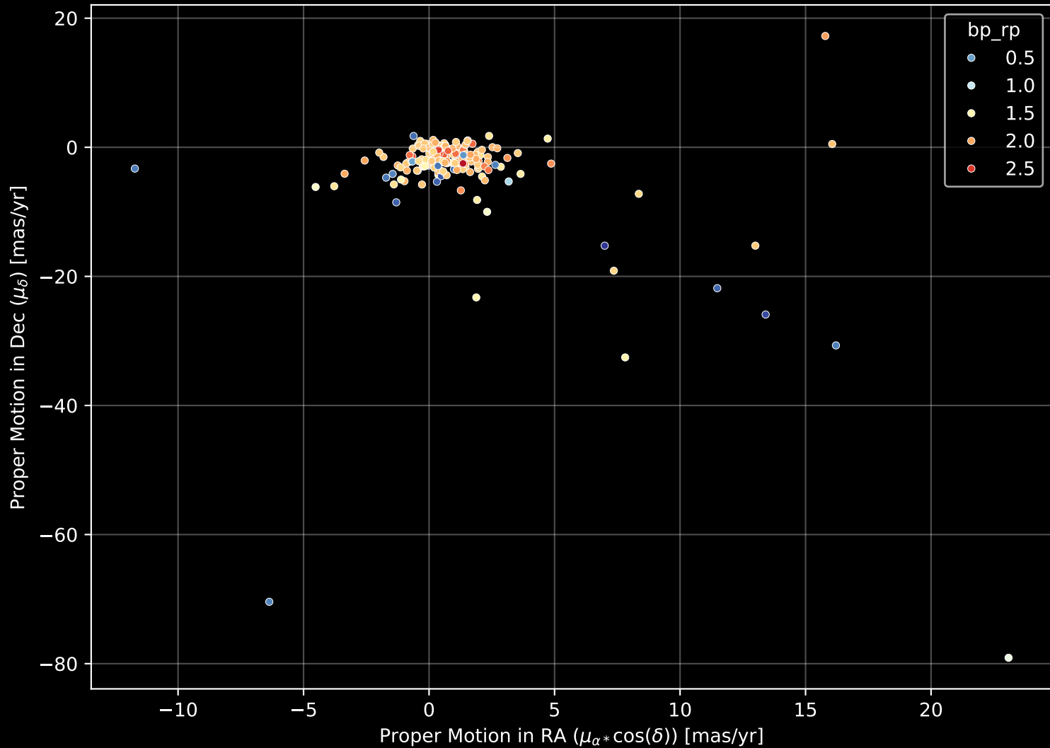
APOGEE DR17 Field: [173-04] Proper Motion Diagram (n= 192)
