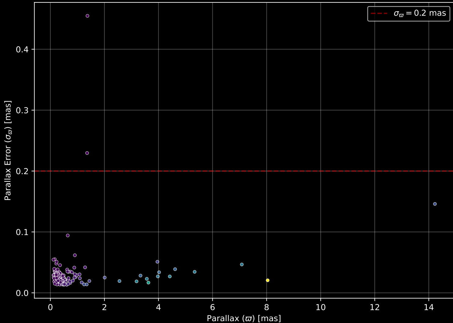
APOGEE DR17 Field: [173-04] Parallax Quality (n= 192)
