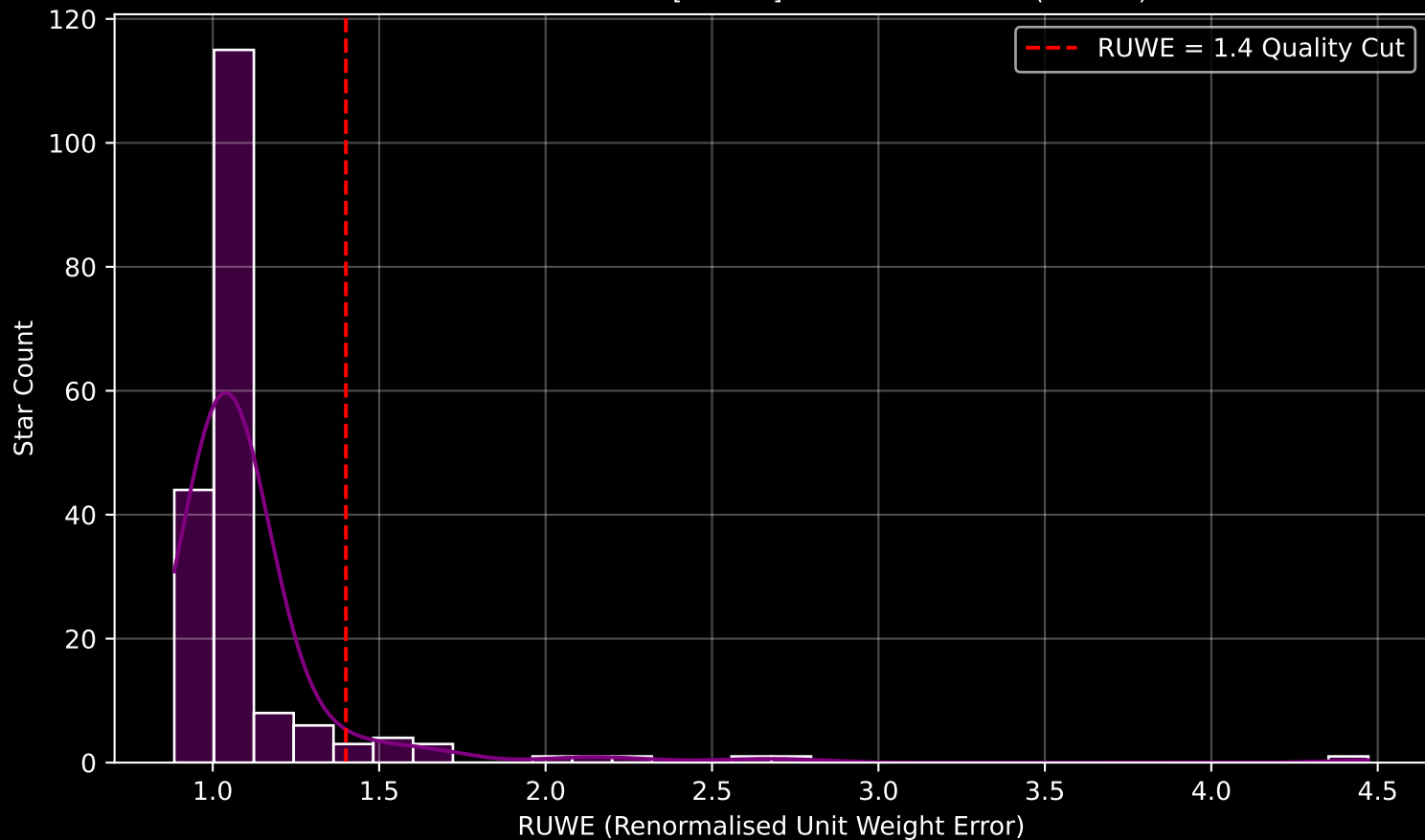
GAPOGEE DR17 Field [173-04] RUWE Distribution (n= 189)
