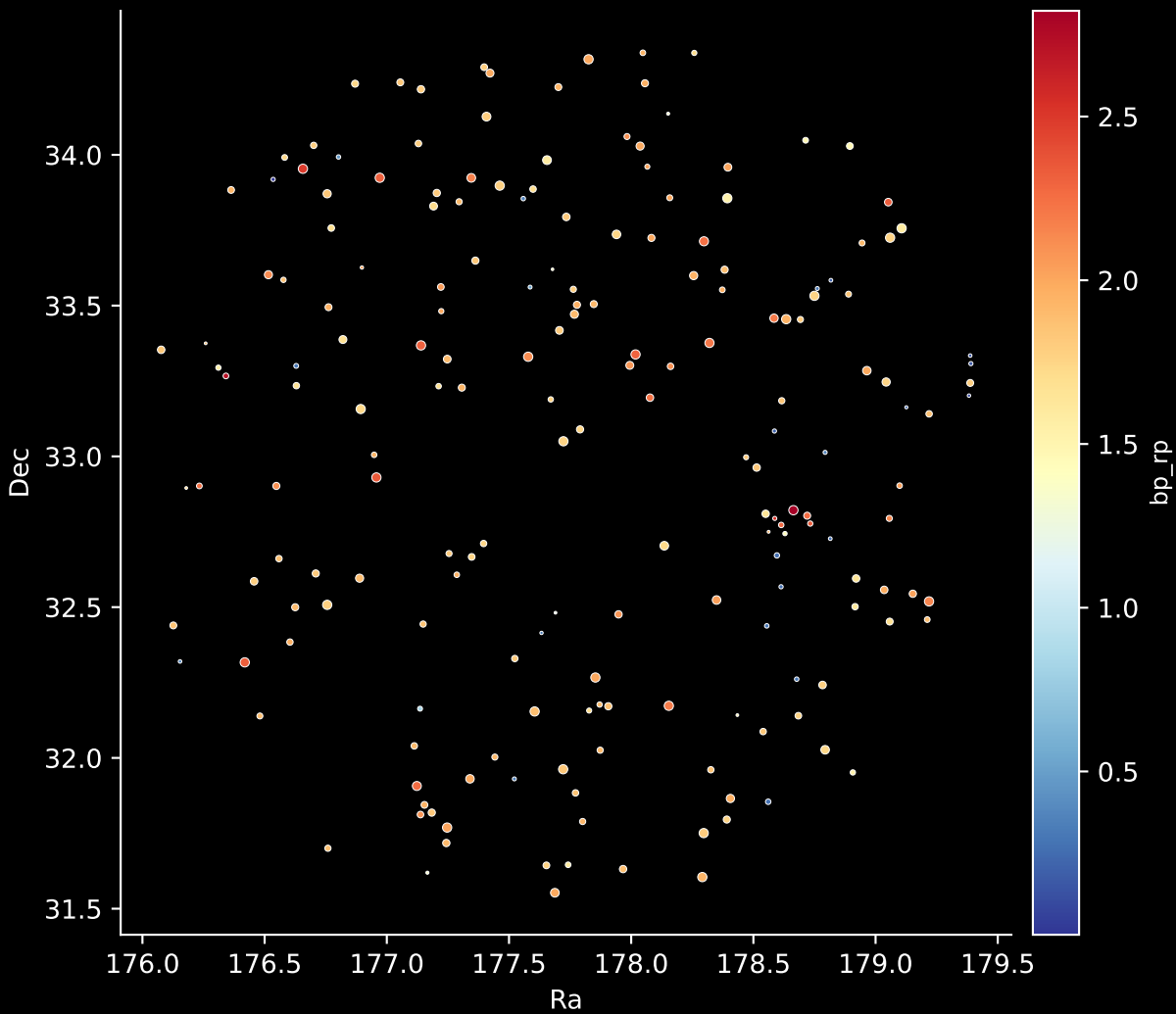
APOGEE DR17 Field: [173-04] Stars: 192
